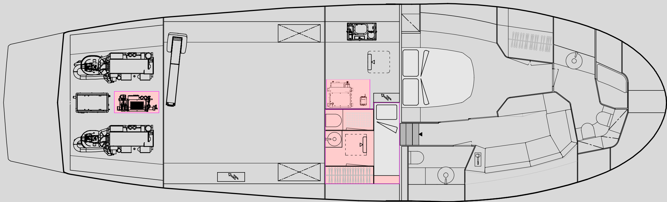
LOWER DECK
