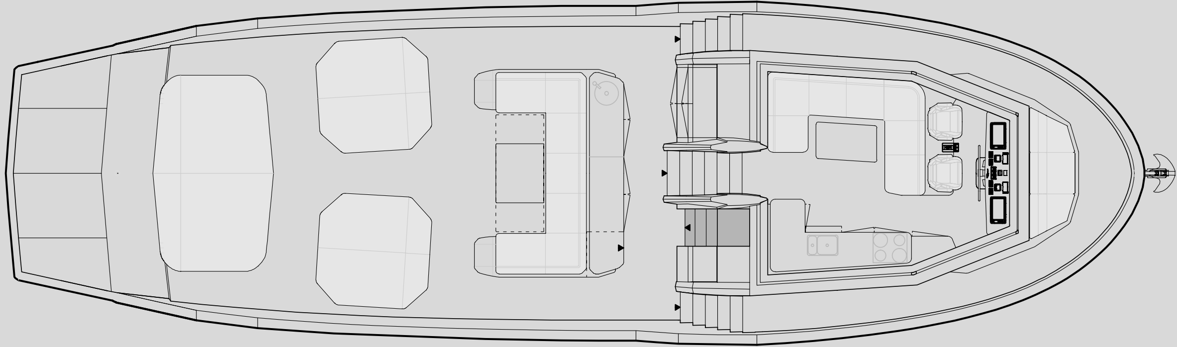
MAIN DECK
