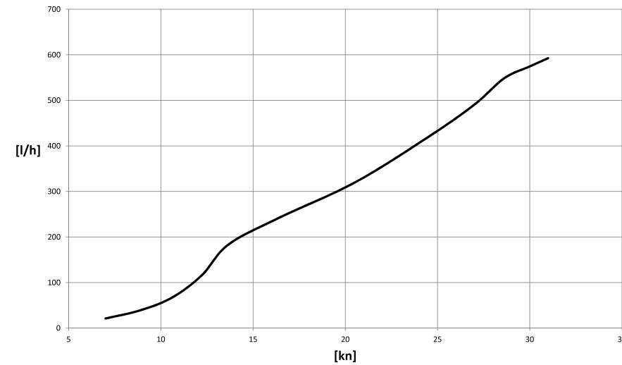
FY780 - 2 x MAN 12V 1550 mhp Fuel consumption [l/h]
