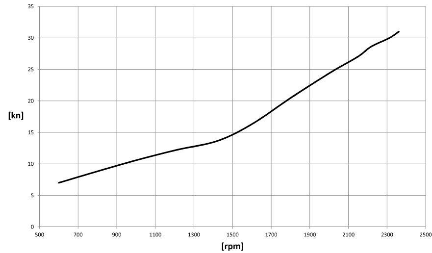
FY780 - 2 x MAN 12V 1550 mhp Speed [kn]
