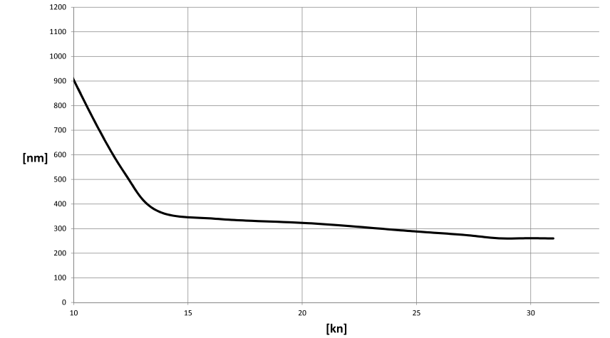
FY780 - 2 x MAN 12V 1550 mhp Range in nm
