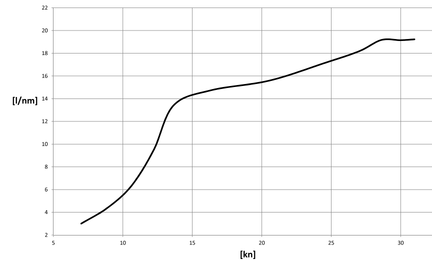
FY780 - 2 x MAN 12V 1550 mhp Fuel consumption [l/nm]
