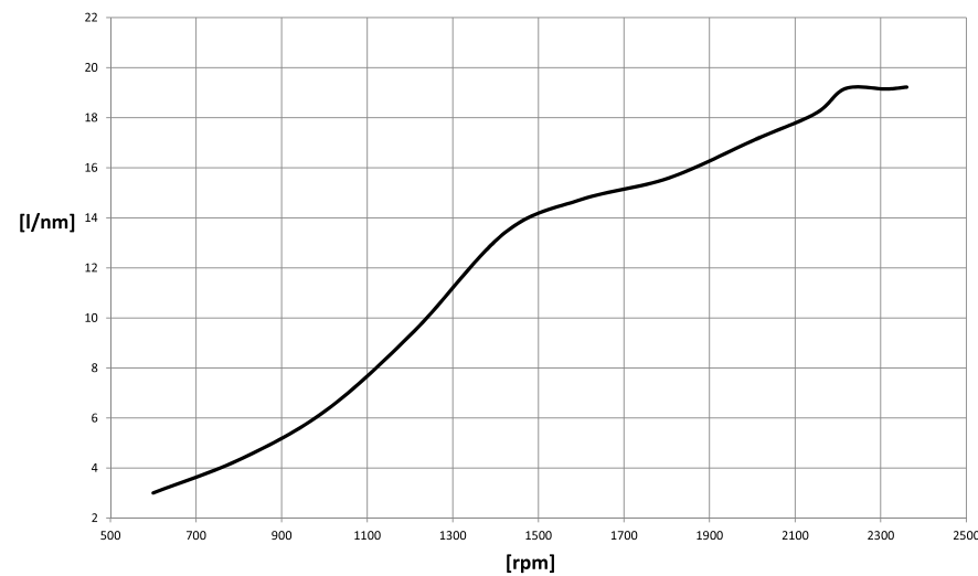
FY780 - 2 x MAN 12V 1550 mhp Fuel consumption [l/nm]
